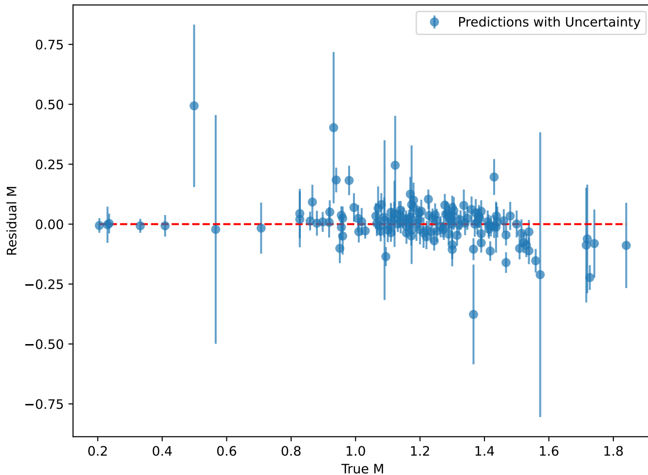
70 Prediction Residuals
