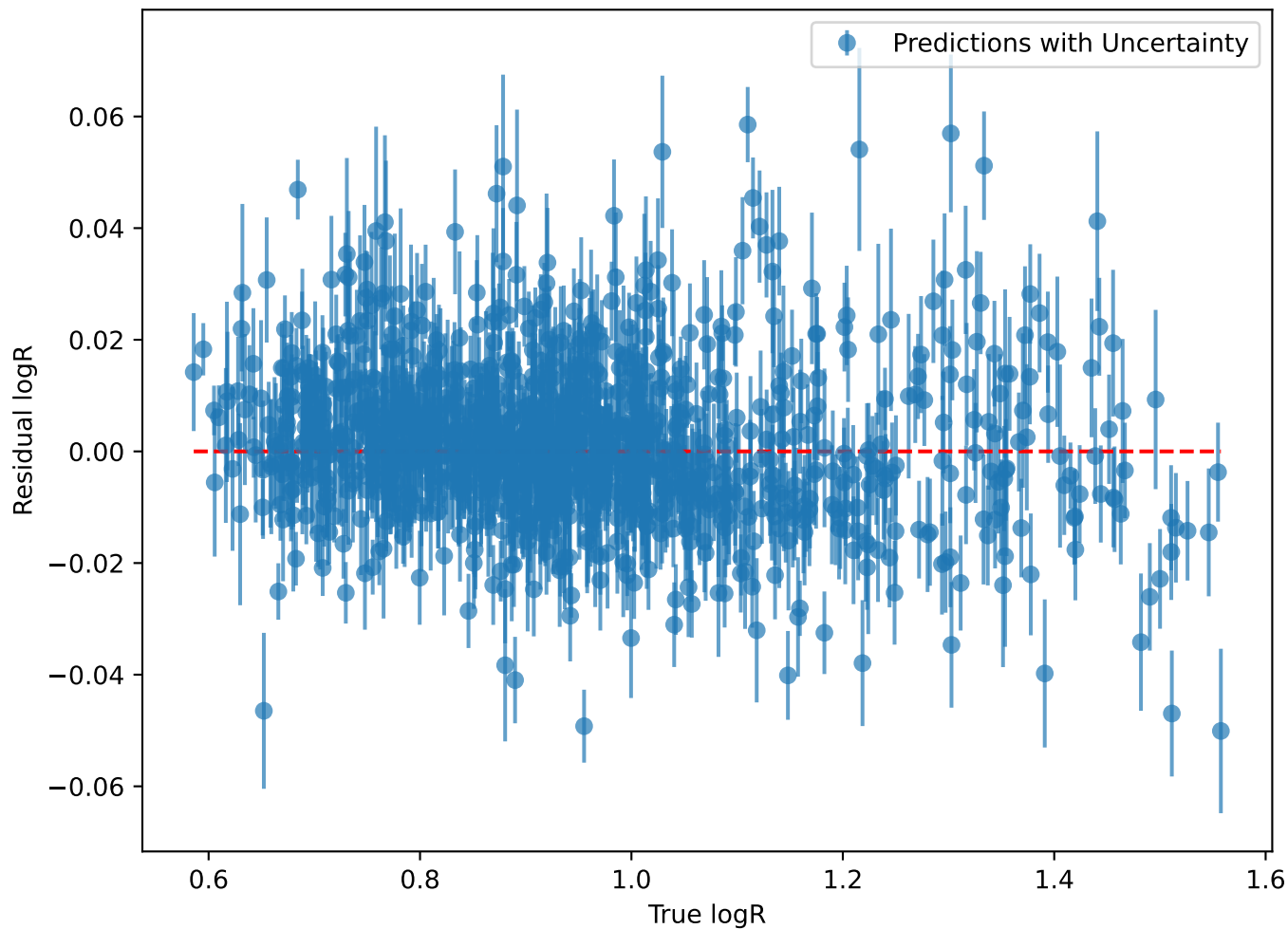
NN Prediction Residuals
