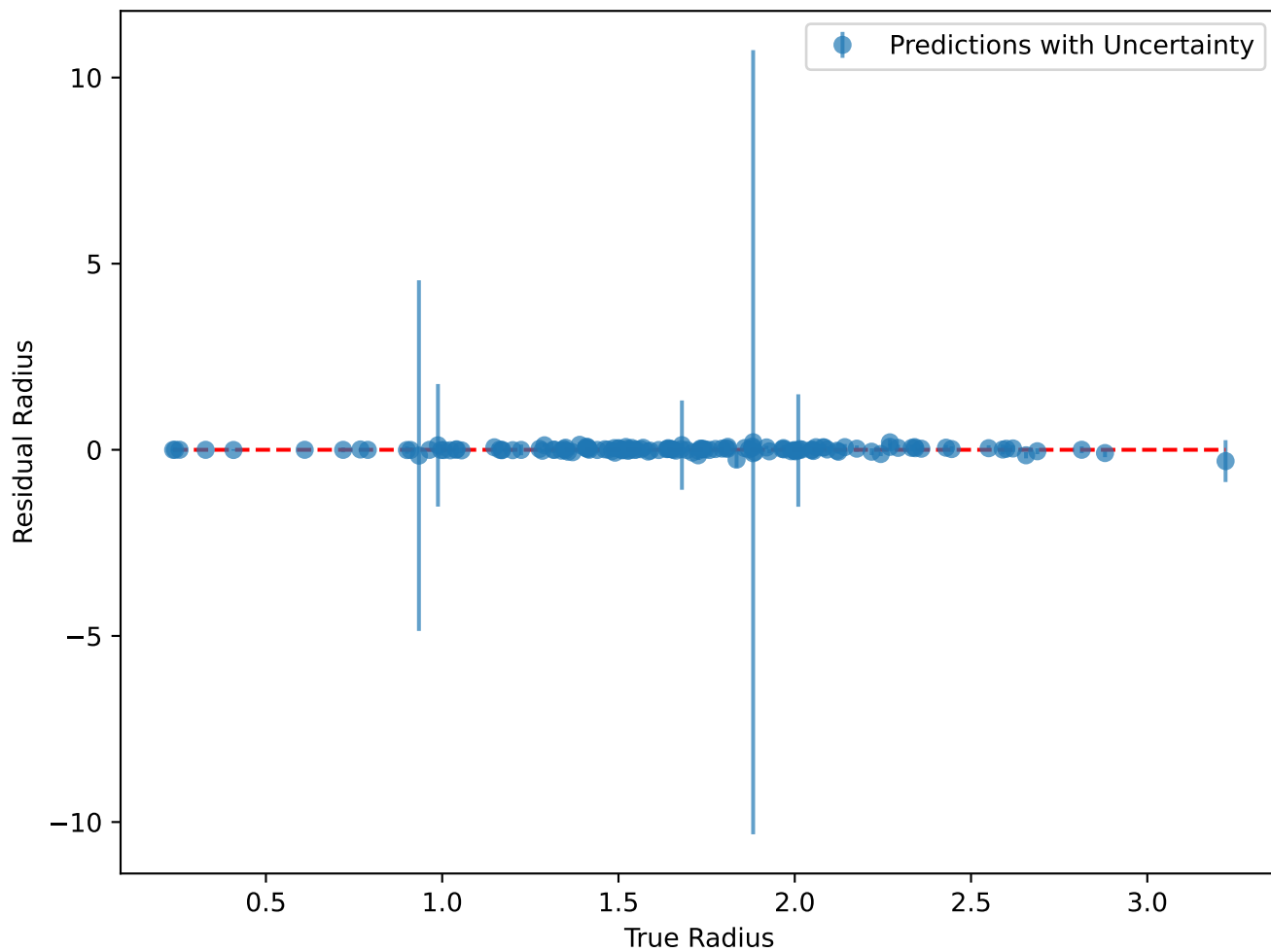
GPrad Prediction Residuals
