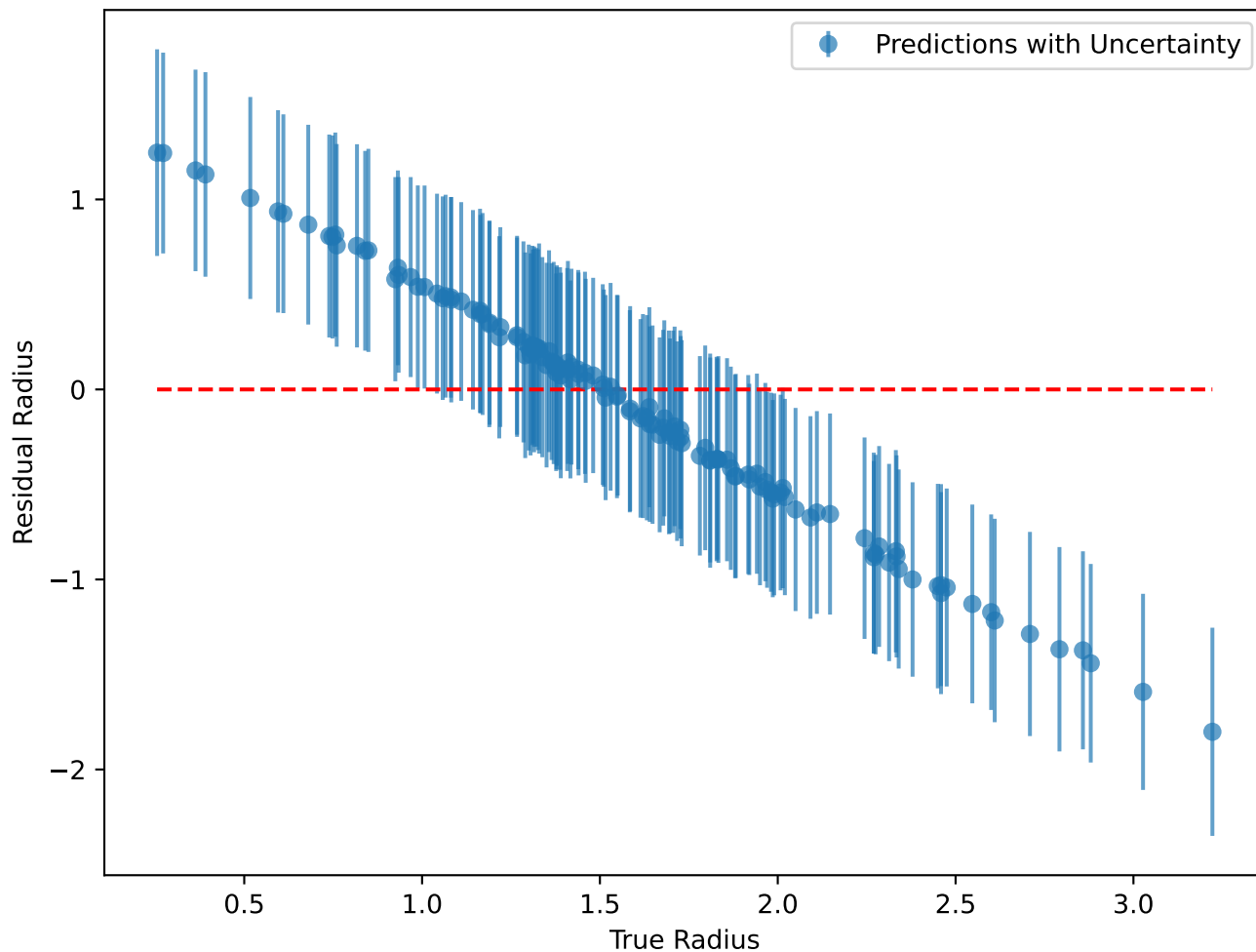
GP Prediction Residuals
