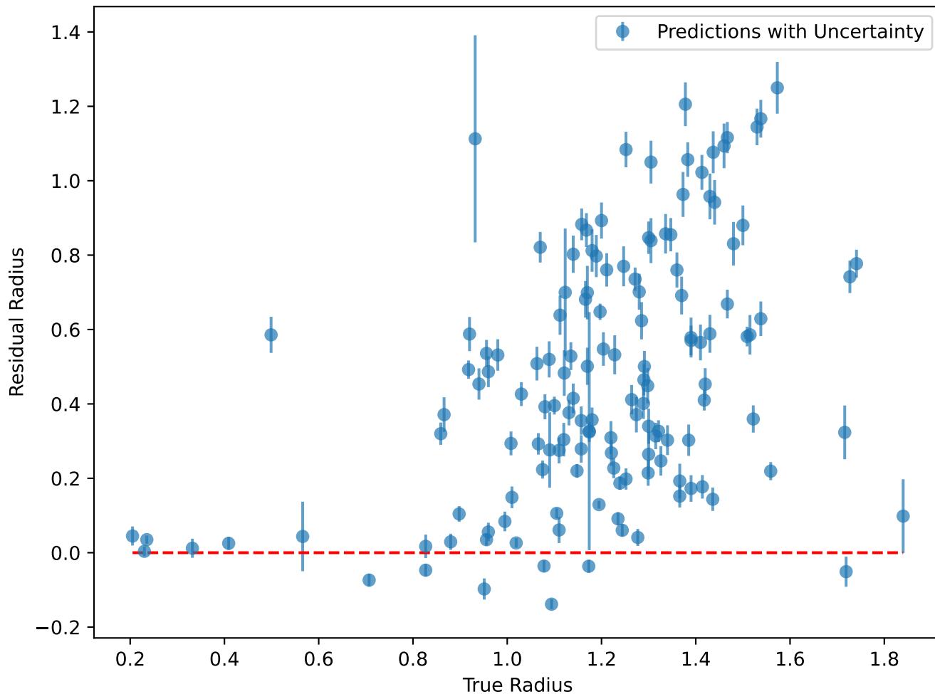
NNrad Prediction Residuals
