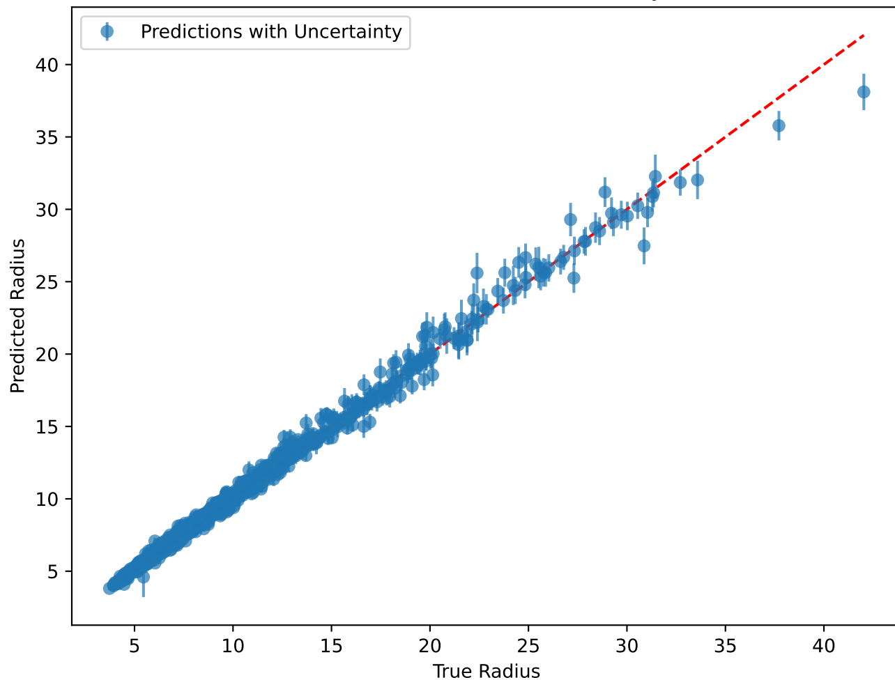
NN Predictions with Uncertainty
