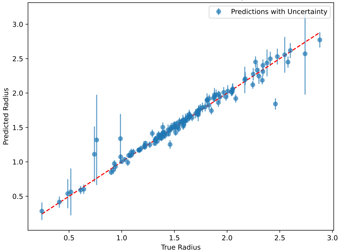
GP Predictions with Uncertainty
