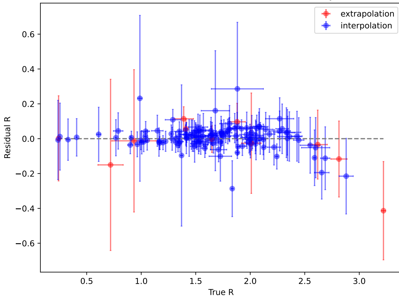
GP Prediction Residuals with Value Uncertainty
