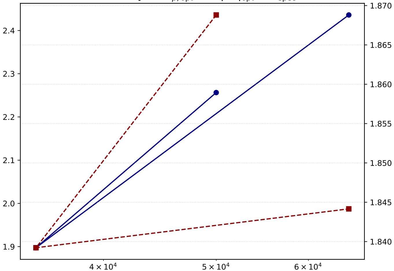
Sensitivity of m_{\rho, \text{opt}} and |\Delta\kappa|_{\text{opt}} to \kappa_{\text{spec}}
