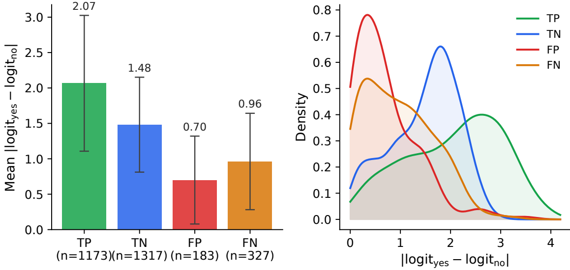
Figure 11: Absolute logit gap |\ell_{yes} - \ell_{no}| at the answer position on the 3,000-question adversarial run. Left: per-category mean with one-standard-deviation error bars (TP n=1173 , TN n=1317 , FP n=183 , FN n=327 ; means 2.07, 1.48, 0.70, 0.96). Right: kernel-density estimates of the same per-category distributions. The order TP > TN > FN > FP at the mean separates confidence from correctness rather than object presence, which is why correction methods that key off uncertainty trade TPs for FNs at about the same rate as FPs for TNs.
