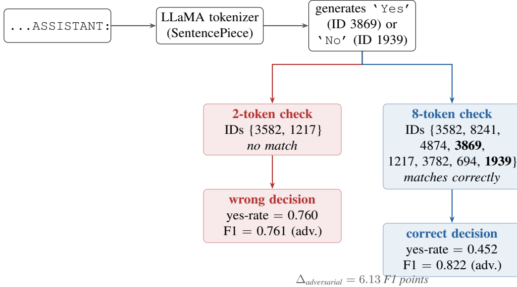
Figure 1: Decision path at the POPE answer position for LLaVA-1.5-7B. The model consistently emits a space-prefixed surface form (‘Yes’ or ‘No’). The two-token check inspects two IDs the model never produces in this context, so every comparison reads two noise-floor logits against each other. Roughly half of the resulting calls go to “yes” by chance, inflating the yes-rate to 0.760 on a 50% positive split.
