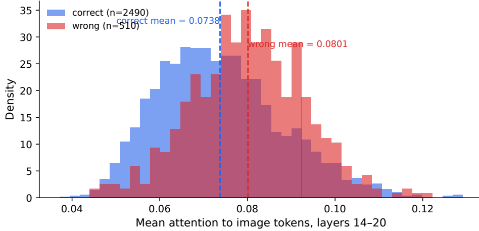
Figure 10: Distribution of mean attention from the final text token to image positions, layers 14–20, on the 3,000-question adversarial run. The blue bars are questions the baseline answered correctly ( n=2490 ); the red bars are wrong ( n=510 ). Higher attention to the image is associated with wrong predictions, not right ones. Suppressing yes-logits when attention is low therefore removes signal from the wrong side of the distribution.
