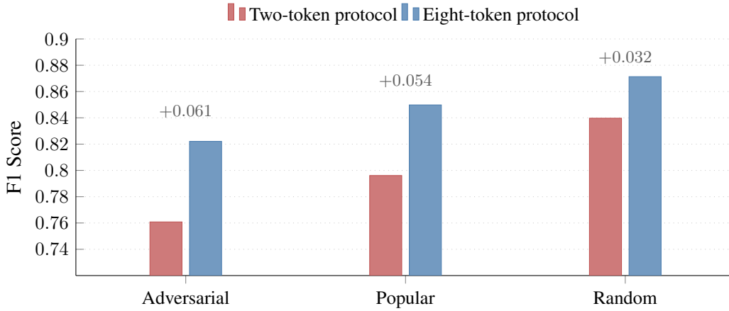
Figure 4: F1 under each protocol across all three splits. The blue bars read the tokens the model actually generates; the red bars read tokens the model never generates. No model or dataset modification is involved.
