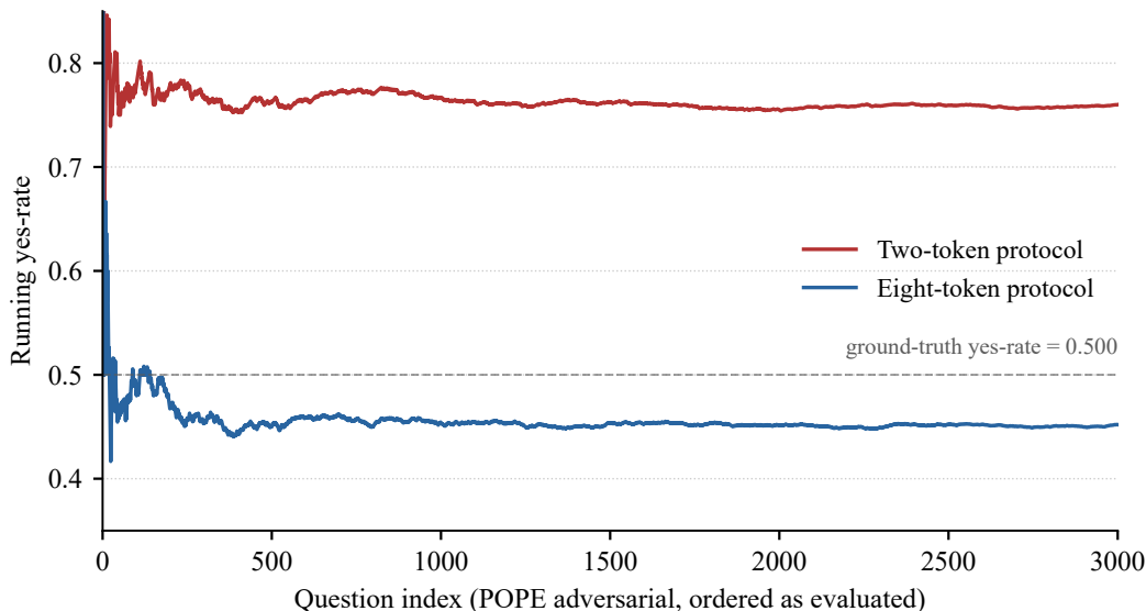
Figure 6: Running yes-rate over the 3,000-question POPE adversarial stream. The eight-token protocol (blue) stabilises near the ground-truth yes-rate (dashed). The two-token protocol (red) stabilises around 0.760 because 56% of true-No questions get mis-labelled when both compared logits are near the vocabulary noise floor.
