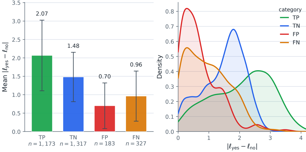
Figure 11: Absolute logit gap |\ell_{\text{yes}} - \ell_{\text{no}}| at the answer position on the 3,000-question adversarial run. Left: per-category mean with one-standard-deviation error bars (TP n=1173 , TN n=1317 , FP n=183 , FN n=327 ; means 2.07, 1.48, 0.70, 0.96). Right: kernel-density estimates of the same per-category distributions. The order \text{TP} > \text{TN} > \text{FN} > \text{FP} at the mean separates confidence from correctness rather than object presence, which is why correction methods that key off uncertainty trade TPs for FNs at about the same rate as FPs for TNs.
