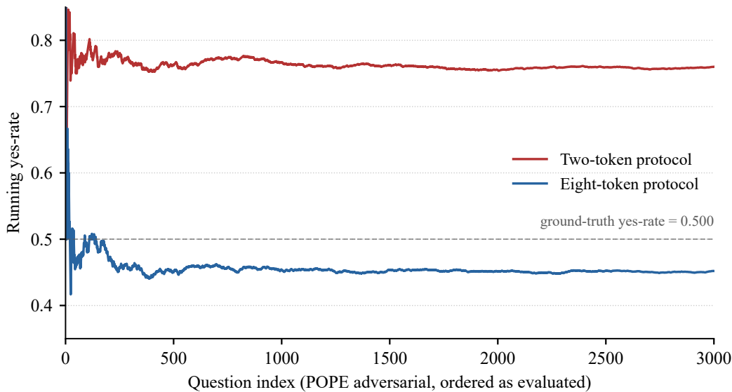
Figure 6: Running yes-rate over the 3,000-question POPE adversarial stream. The eight-token protocol (blue) stabilises near the ground-truth yes-rate (dashed). The two-token protocol (red) stabilises around 0.760 because 56% of true-No questions get mis-labelled when both compared logits are near the vocabulary noise floor.
