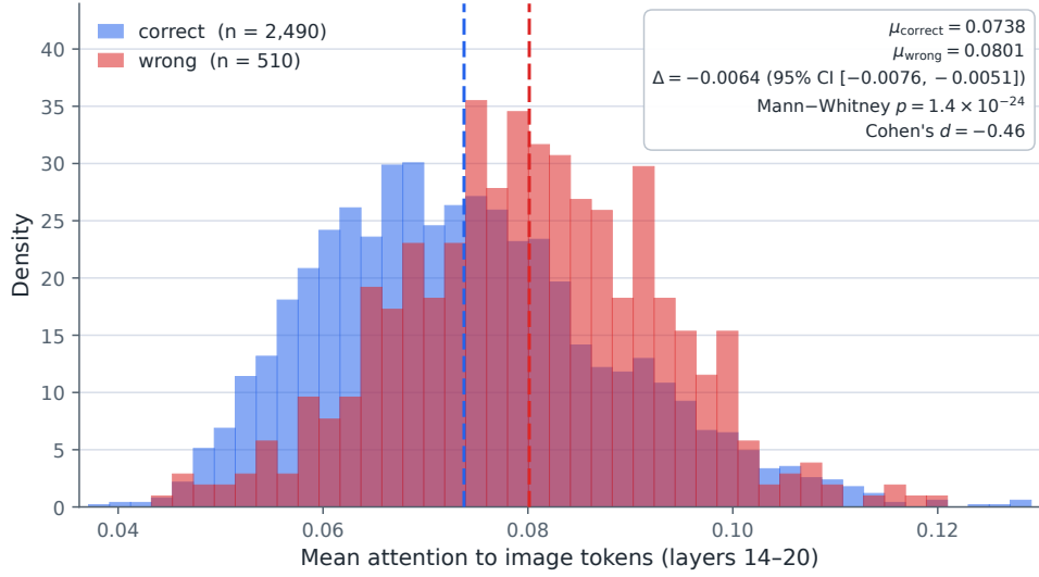
Figure 10: Distribution of mean attention from the final text token to image positions, layers 14–20, on the 3,000-question adversarial run. The blue bars are questions the baseline answered correctly ( n=2490 ); the red bars are wrong ( n=510 ). Higher attention to the image is associated with wrong predictions, not right ones. Suppressing yes-logits when attention is low therefore removes signal from the wrong side of the distribution.
