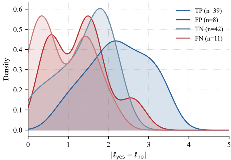
Logit-gap density by category
