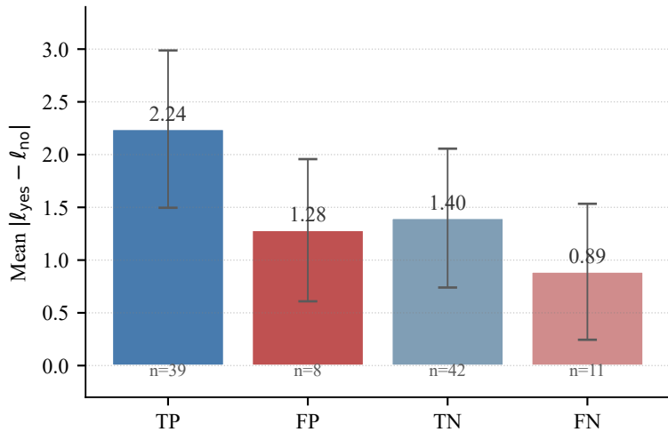
Per-category mean logit gap
