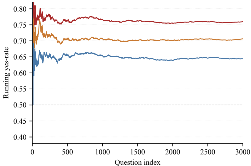
Two-token protocol
