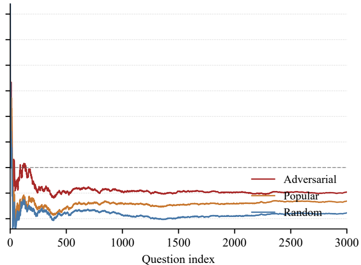
Eight-token protocol
