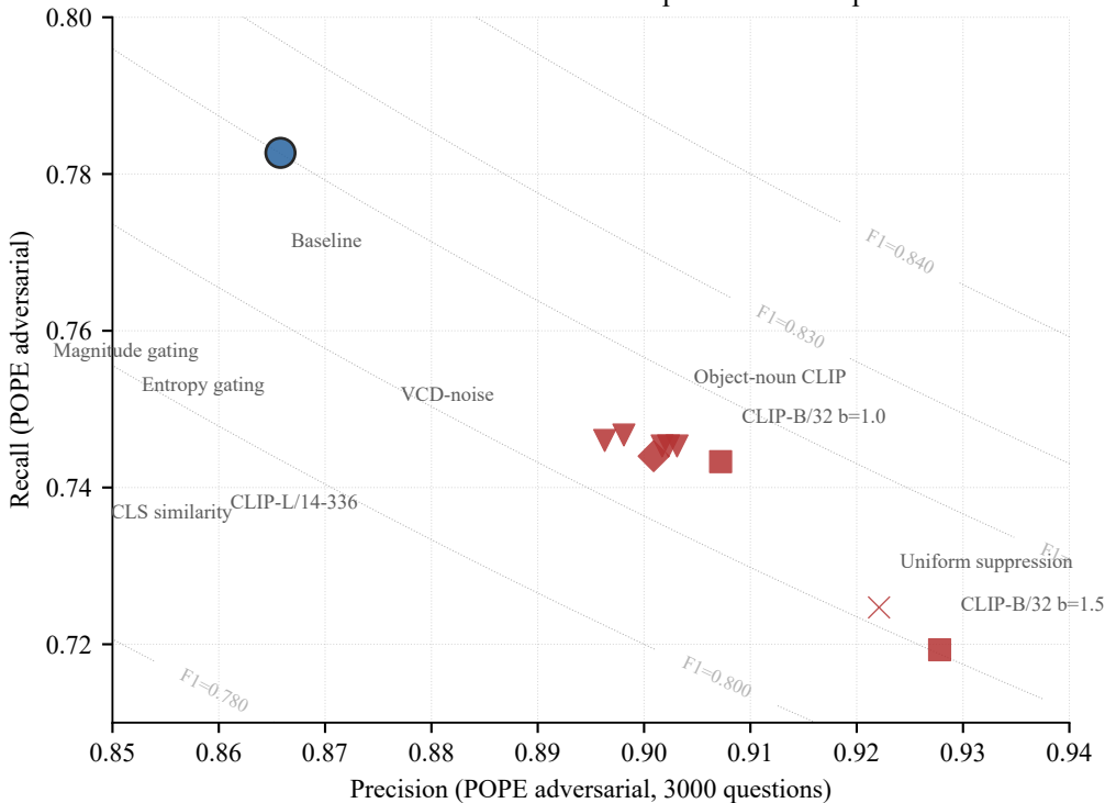
Inference-time corrections on the precision-recall plane
