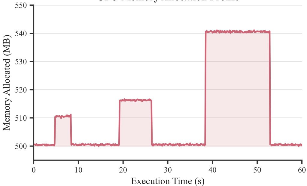
GPU Memory Allocation Profile
