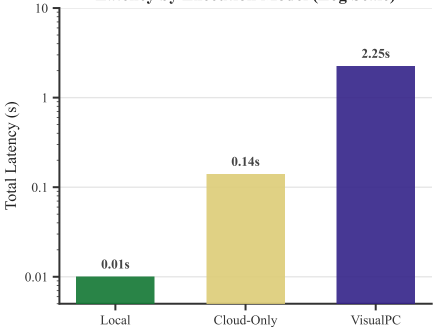
Latency by Execution Model (Log Scale)
