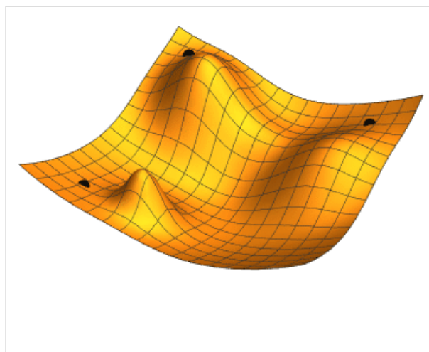
Illustration of gradient descent for three different starting points; two parameters (represented by the plan coordinates) are adjusted in order to minimize the loss function (the height). [76]
