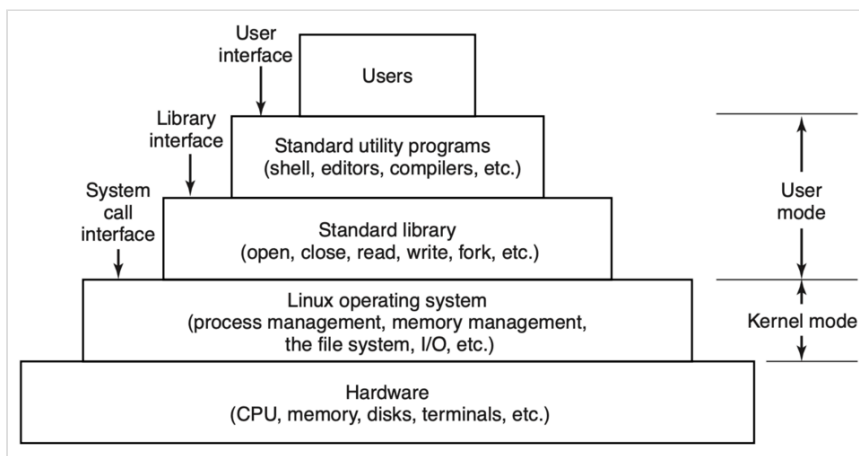
Layers of a Linux system
