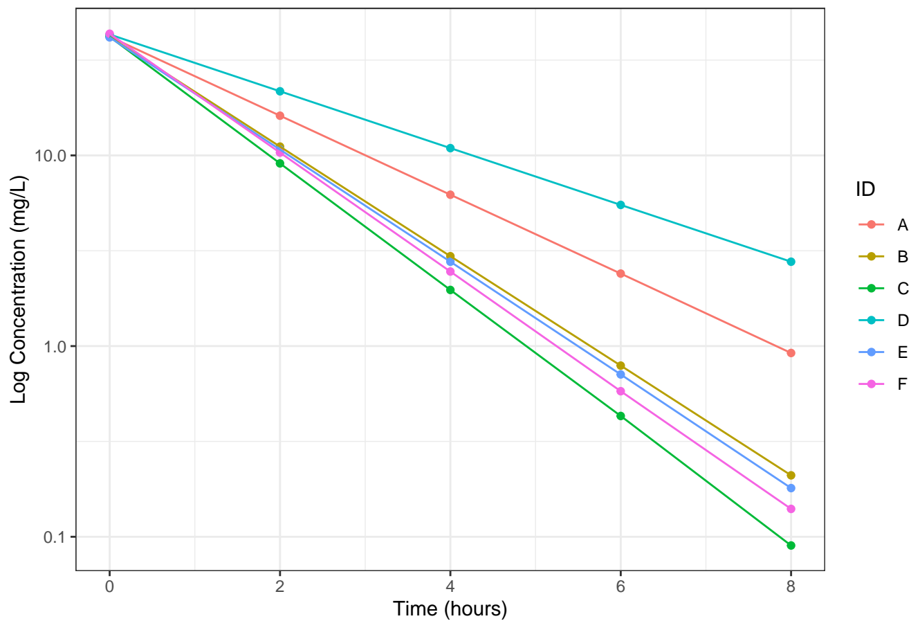
Log-Scale Concentration–Time Profiles
