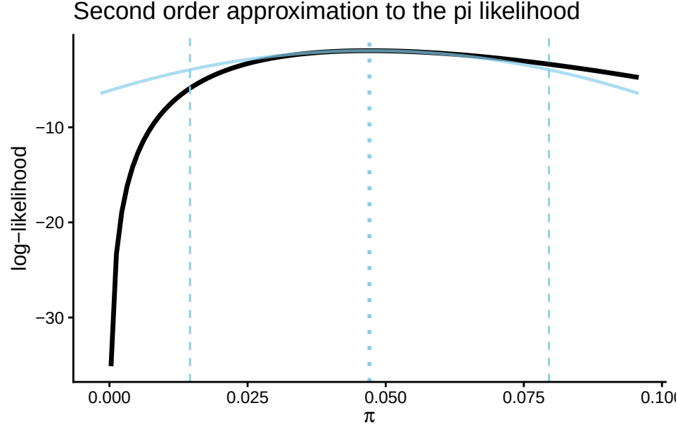
Figure 2: Log-likelihood function and second-order approximation for pi.
