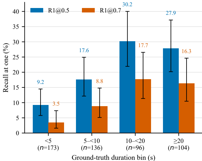
(a) Top-1 localization performance
