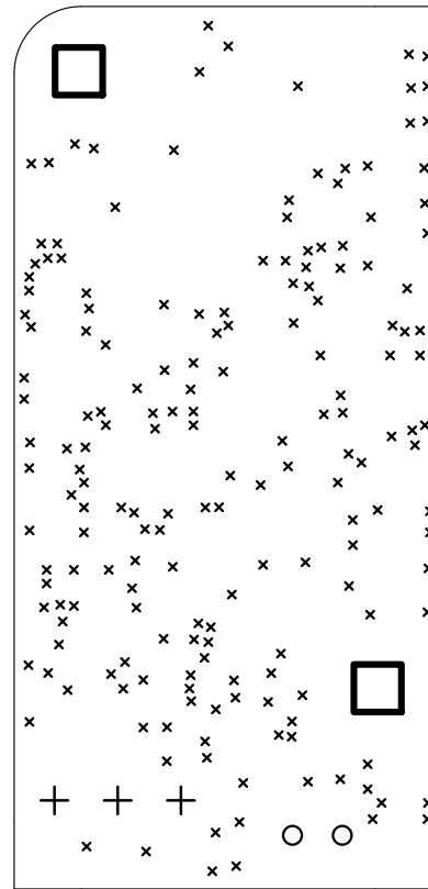
Drill Map:
