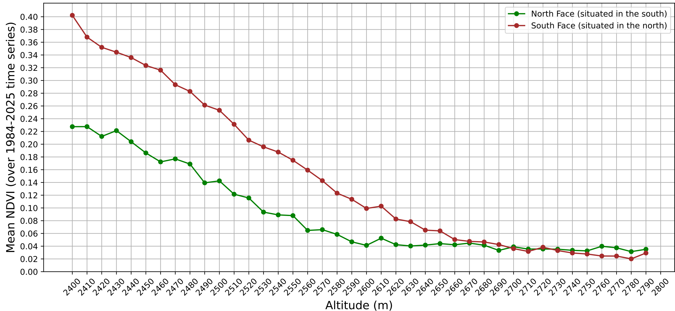
NDVI mean vs altitude — South Face vs North Face (10m intervals)
