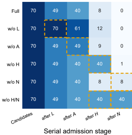
(a) Stagewise retention
