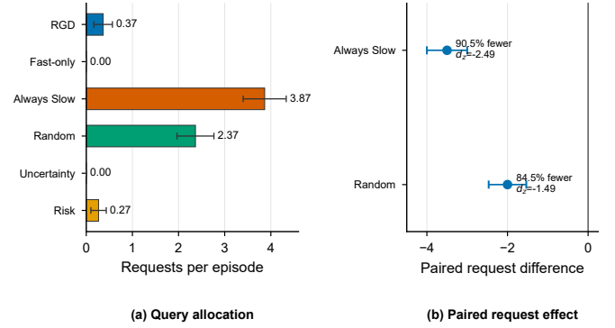
Fig. 4. Slow-path allocation under the 30-seed protocol. (a) Mean requests per episode with 95% seed-bootstrap intervals. (b) RGD-minus-baseline differences for the two request-intensive allocators. Negative values denote fewer RGD requests.
