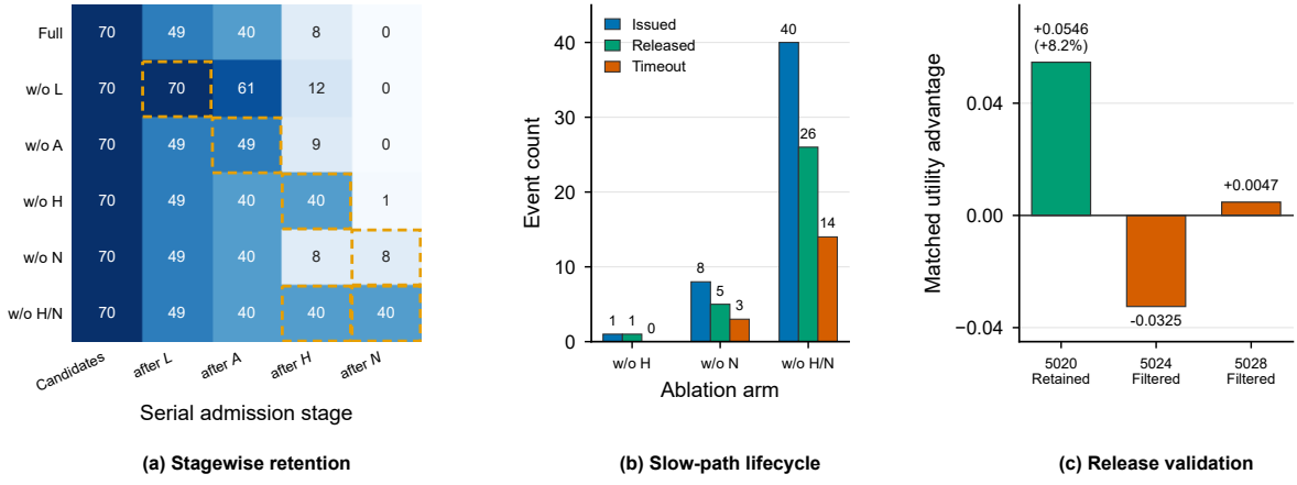
Fig. 8. Six-condition gate ablation and matched-proposal release audit. (a) Serial candidate retention. Dashed cells mark omitted predicates. (b) Issued, released, and timed-out requests over 20 seeds. (c) Matched-rollout utility advantage for the three post-projection distinct interventions. Horizontal labels are seed identifiers, and retained and filtered denote the release-validation outcome.
