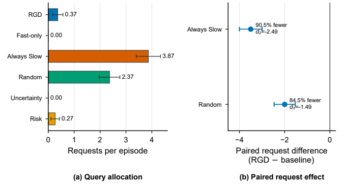
Fig. 4. Slow-path allocation under the 30-seed paired protocol. (a) Mean requests per episode with 95% seed-bootstrap intervals. (b) Paired RGD-minus-baseline differences for the two request-intensive allocators; negative values denote fewer RGD requests.
