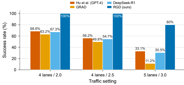
Fig. 3. Success rates across the three highway-env traffic settings of Hu et al. [27].
