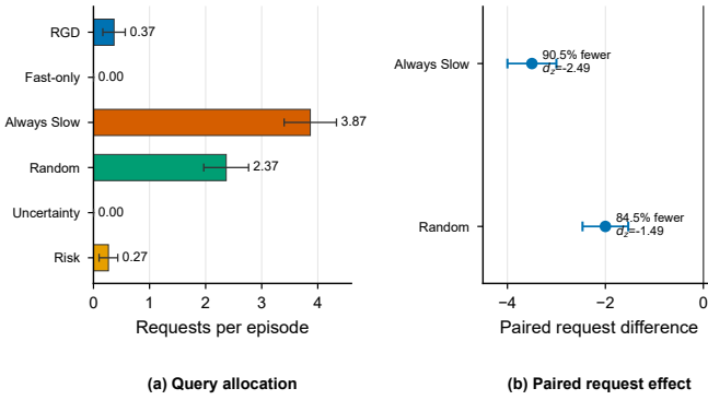
Fig. 4. Slow-path allocation under the 30-seed paired protocol. (a) Mean requests per episode with 95% seed-bootstrap intervals. (b) Paired RGD-minus-baseline differences for the two request-intensive allocators. Negative values denote fewer RGD requests.
