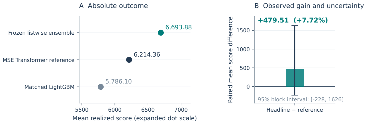
Figure 4: Absolute score is displayed on an expanded dot scale. The gain bar starts at zero and carries the paired seven-day block interval. The point estimate is an observed improvement on this period; the interval represents uncertainty conditional on these records and does not correct historical selection.
