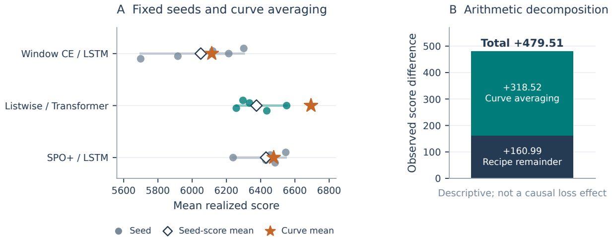
Figure 6: Fixed-seed outcomes, their arithmetic mean, and the curve-mean outcome. Slight vertical offsets in the left panel only separate overlapping markers and carry no quantity. The right panel decomposes the headline-reference difference around the mean single-seed score. It is an arithmetic identity, not an isolated causal effect of the loss or of every implementation change.
