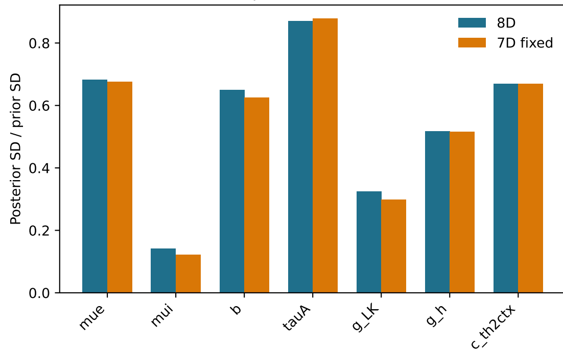
Shared-parameter contraction
