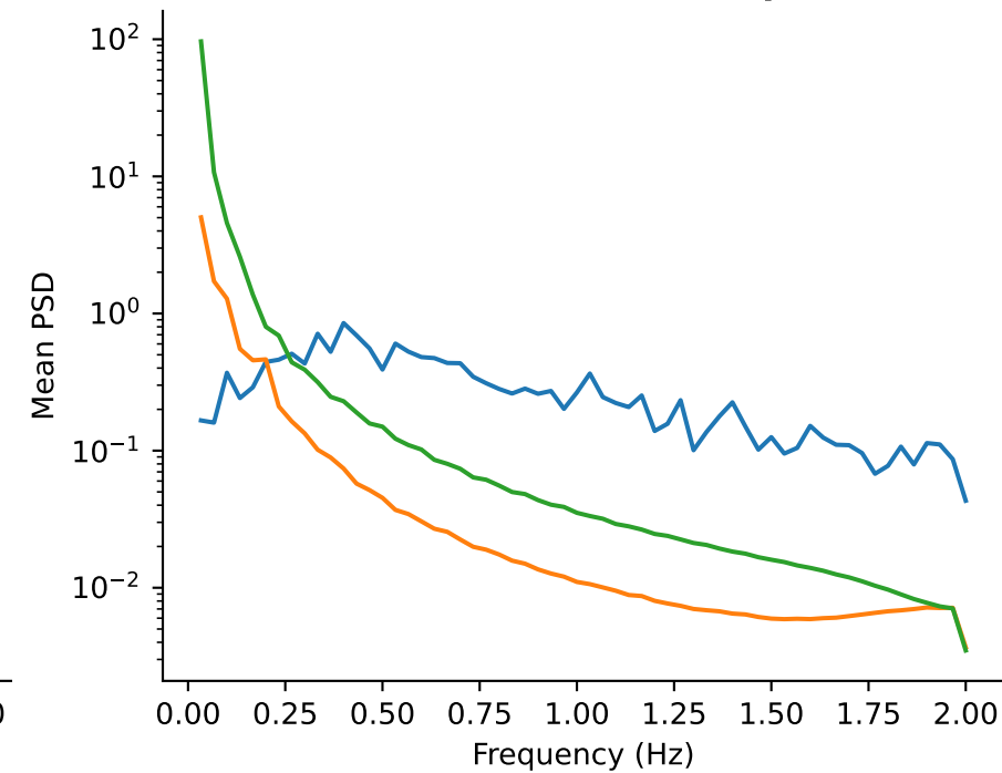
Standardized innovation spectrum
