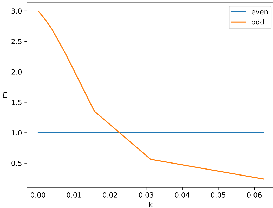
GaussianWell,d=4
