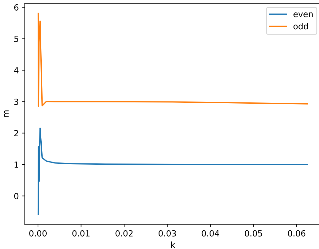
GaussianWell,d=6
