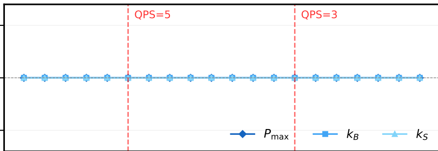
Workload-Adaptive Parameters (online partial fit)
