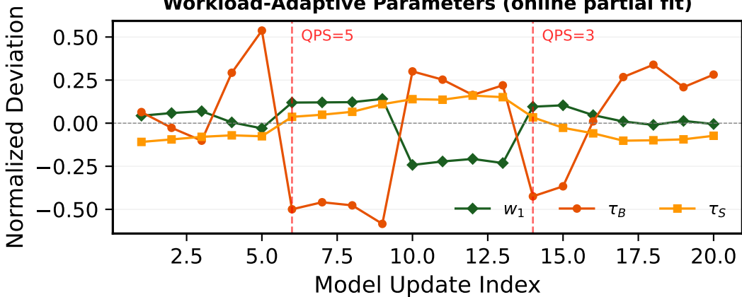
Workload-Adaptive Parameters (online partial fit)
