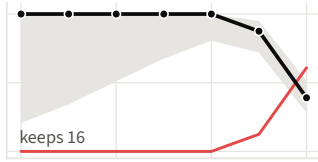
Qwen3.8-27B
