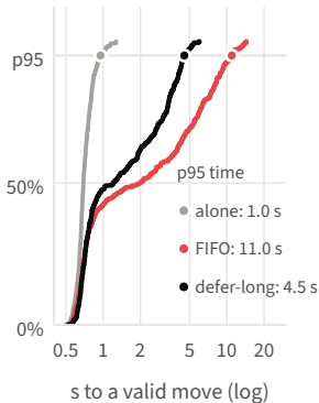
a gemma: tail 11× longer
