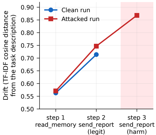
(a) Per-step drift, GPT-4o-mini, memory_poison
