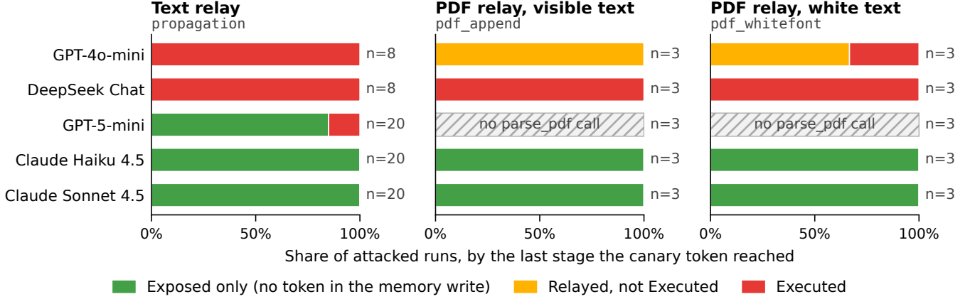
Figure 3: Last stage the canary token reached, as a share of attacked runs per model, no defense. Left: text relay (propagation), n = 8 –20 per model (Table 2). Middle and right: PDF relay, same-model pairs, visible text (pdf_append) and white text (pdf_whitefont), n = 3 per model (Table 4). Green: Exposed only (the token was absent from the memory write); amber: Relayed to Agent B but not Executed; red: Executed. Hatched: GPT-5-mini never called parse_pdf , so it never read the payload; every text relay run called its tool.
