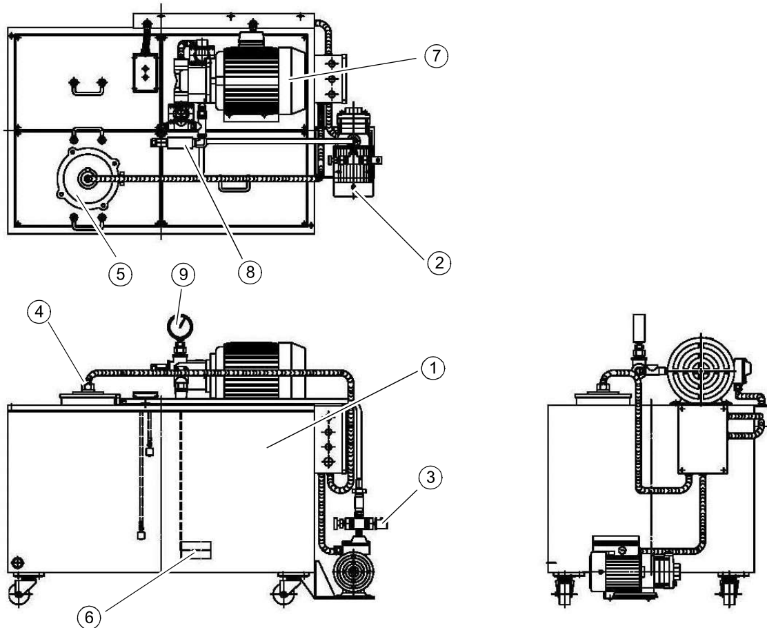
1-1: Externes Kühlaggregat - External cooling unit
