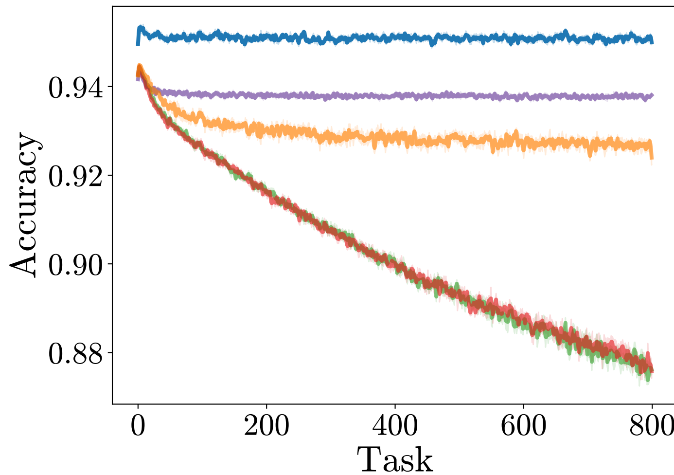
Permuted MNIST
