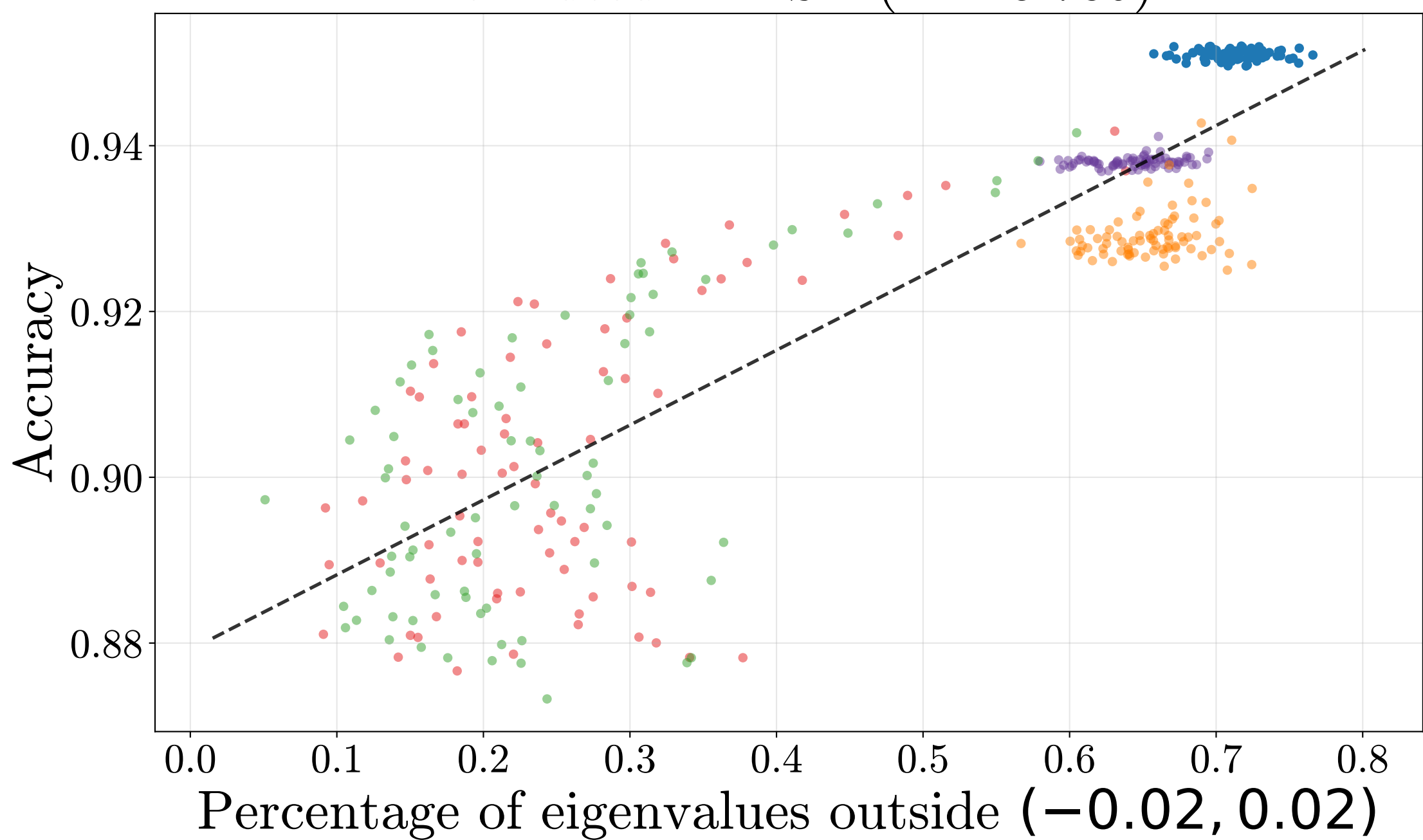
Permuted MNIST ( R^2=0.785 )
