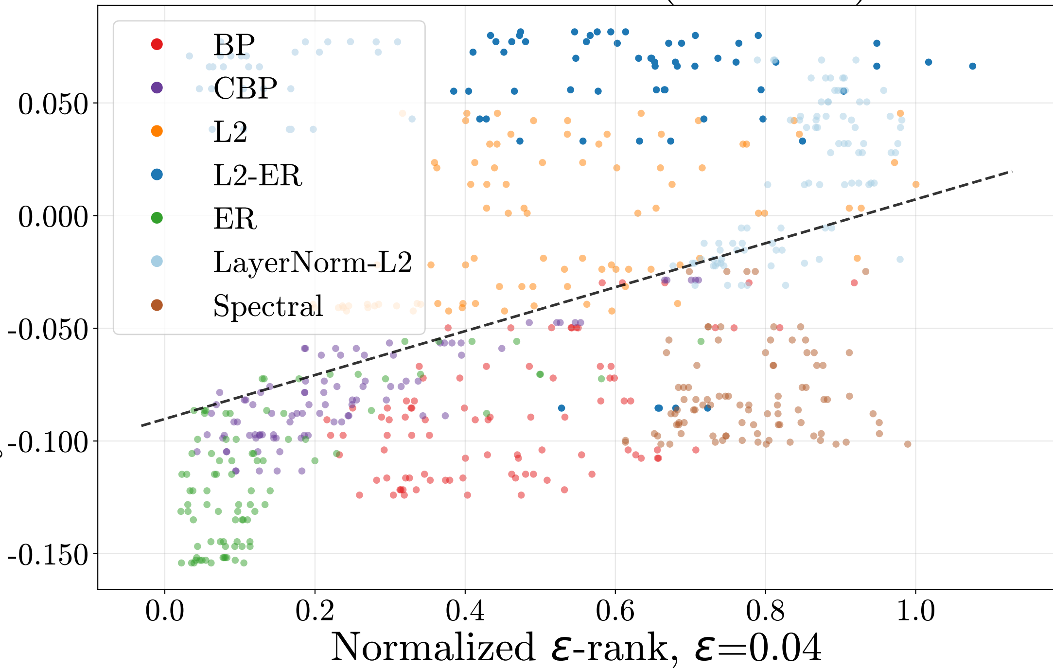
Incremental CIFAR ( R^2=0.182 )
