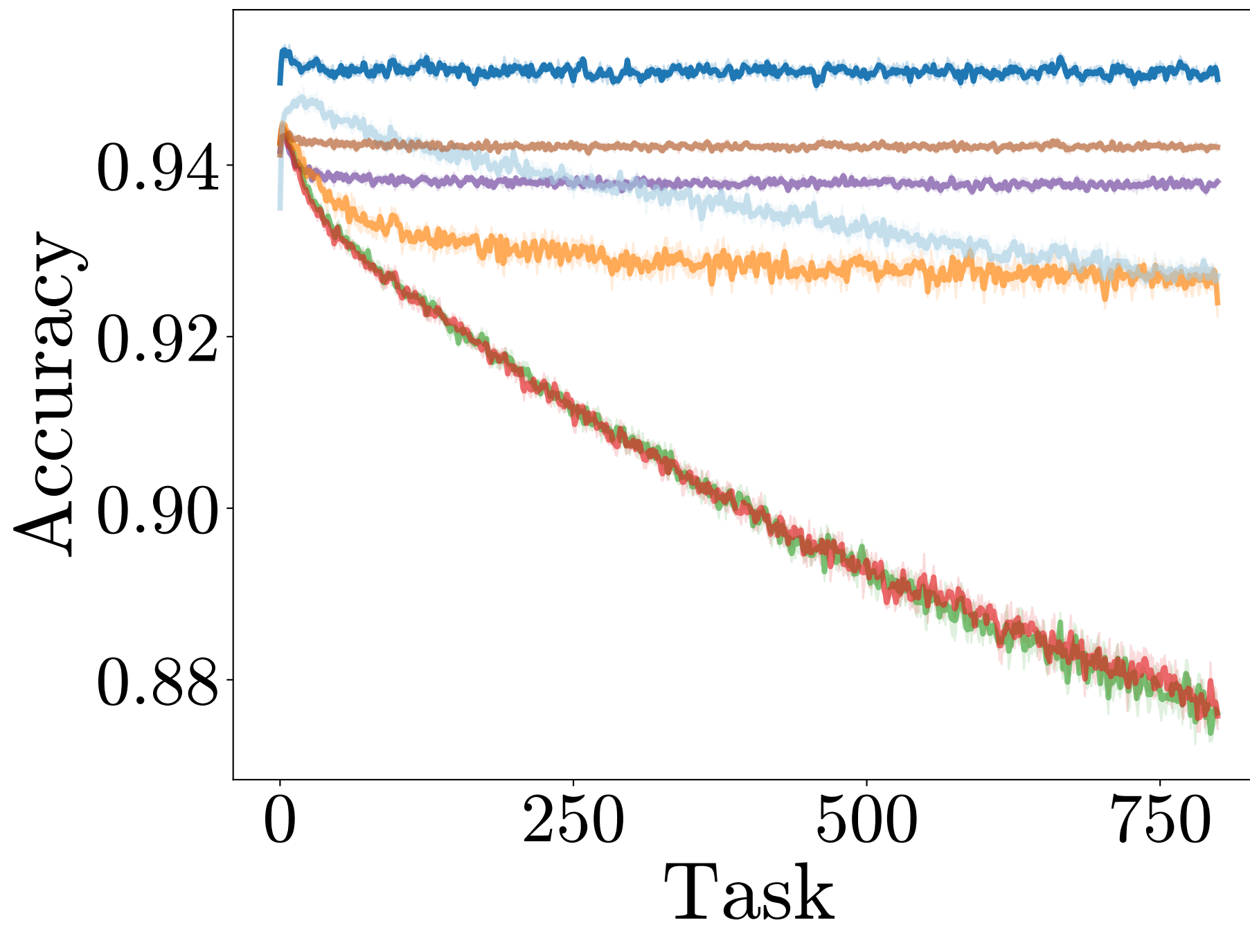
Permuted MNIST
