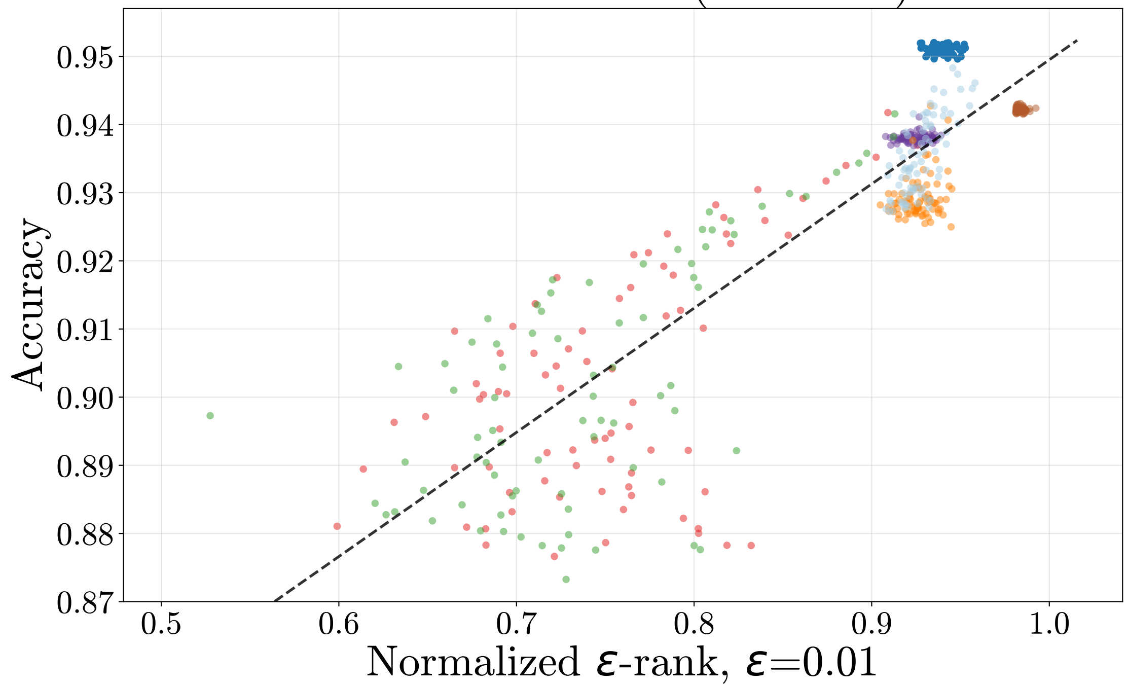
Permuted MNIST ( R^2=0.771 )
