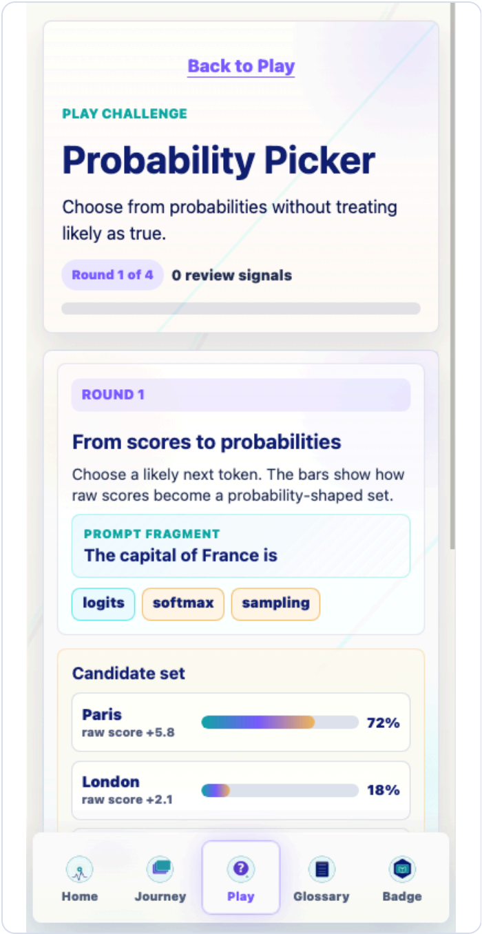
Probability Picker active start at 390px
