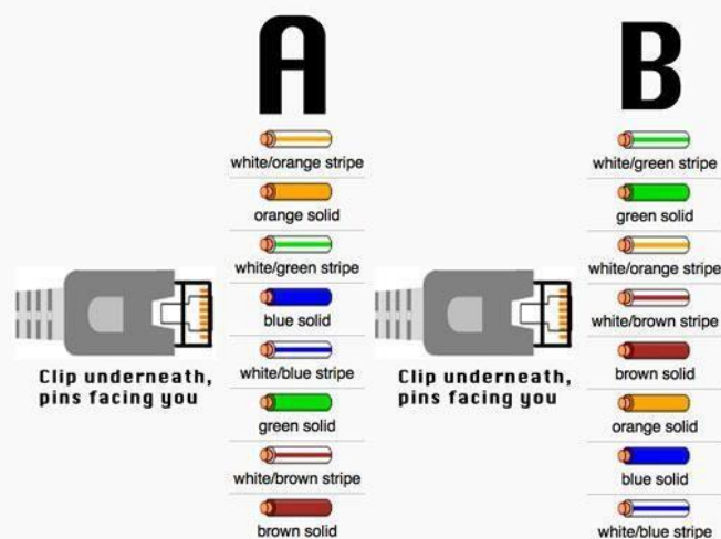
Fig. 2 — T568A / T568B wire colour arrangement used at each end
