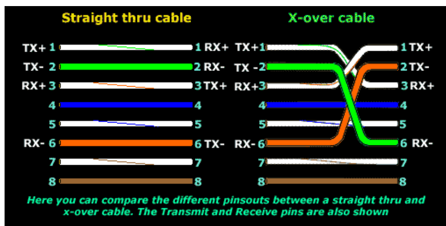
Fig. 1 — Difference between straight-through and crossover pinouts (TX/RX mapping)
