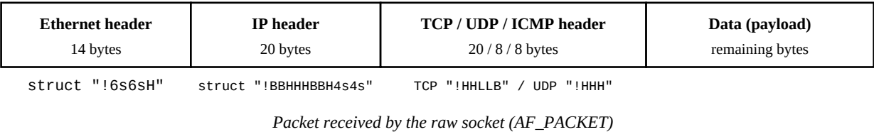
Fig 1: Structure of a captured frame and the struct format used for each header
