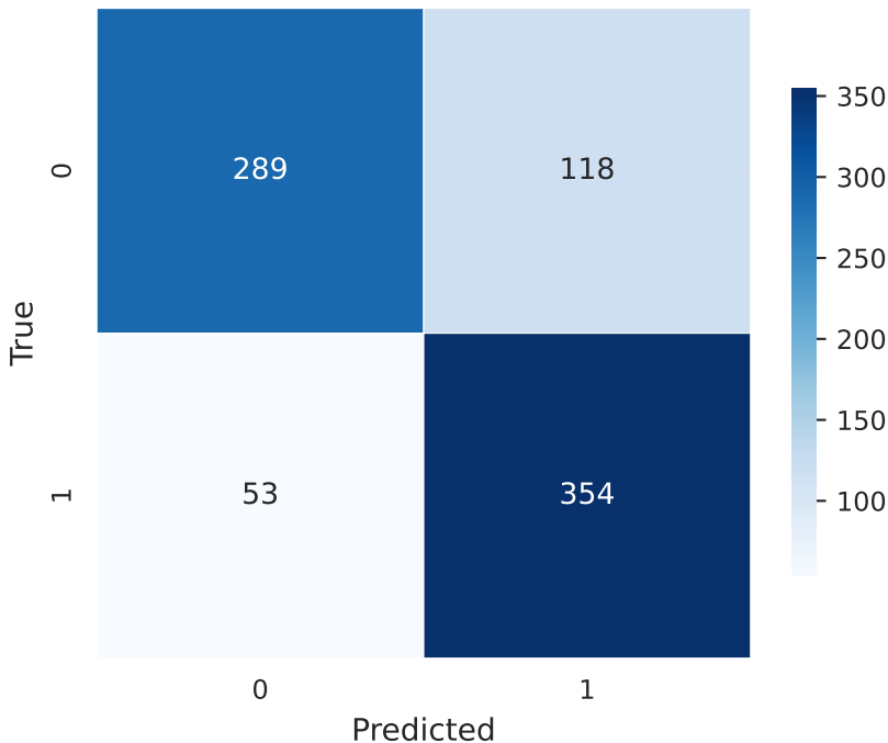
Confusion Matrix - gte-base
