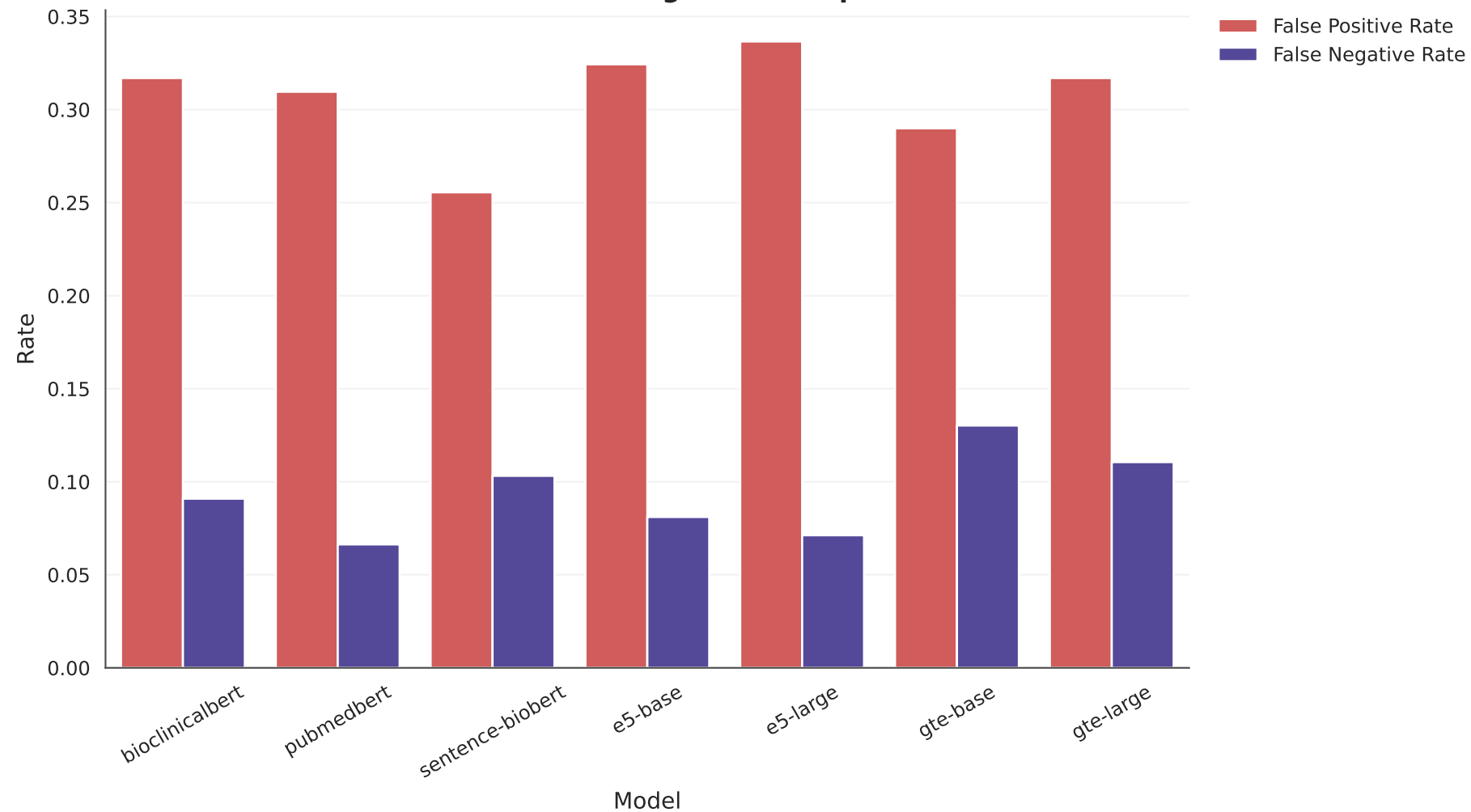
False Positive / False Negative Rate per Model
