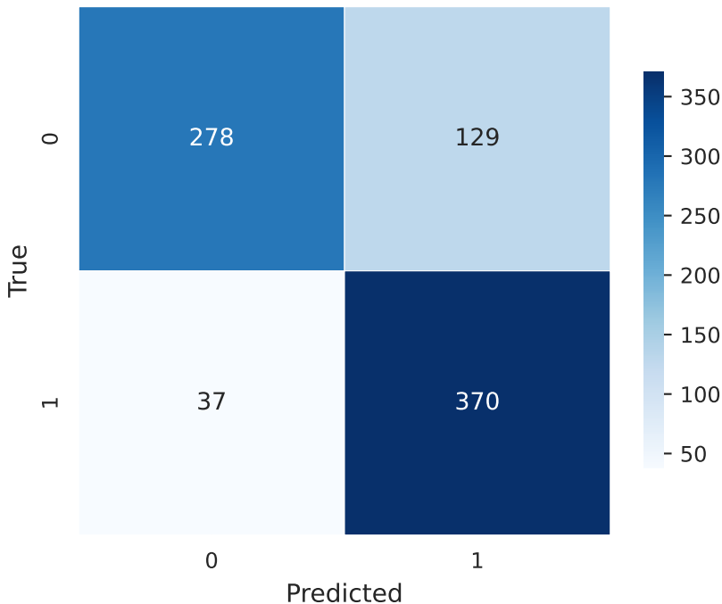
Confusion Matrix - bioclinicalbert
