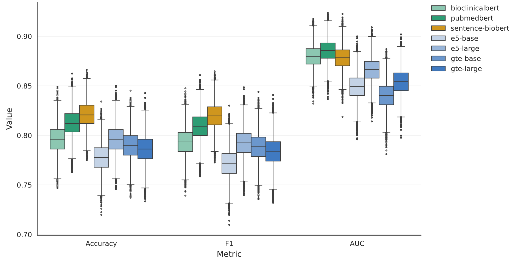
Bootstrap (10k) Metric Distribution per Model
